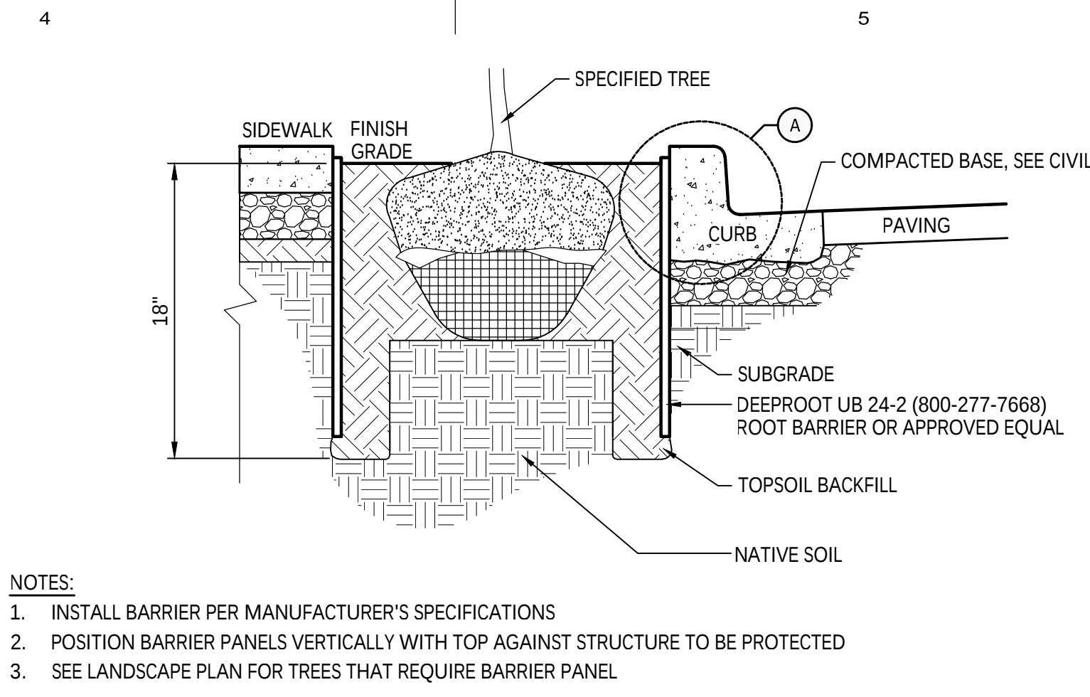
1 ROOT BARRIER Section NOT TO SCALE
