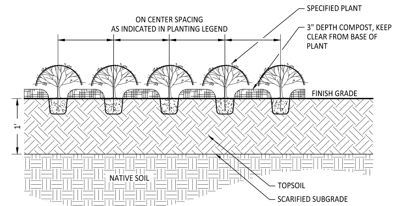
6 GROUNDCOVER PLANTING Section NOT TO SCALE
