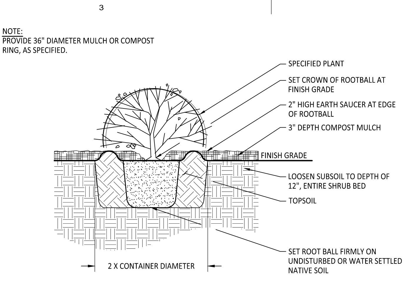
5 SHRUB PLANTING Section NOT TO SCALE
