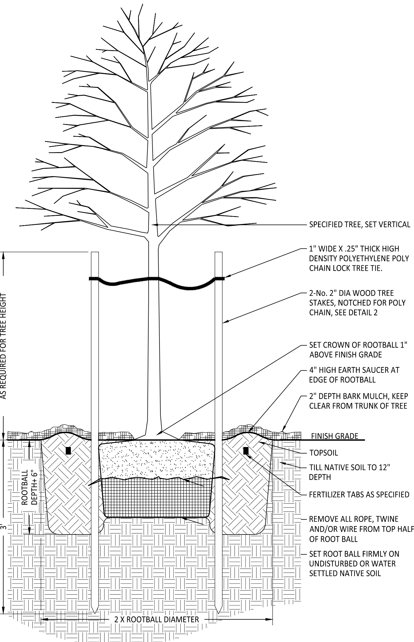
4 DECIDUOUS TREE PLANTING Section NOT TO SCALE
