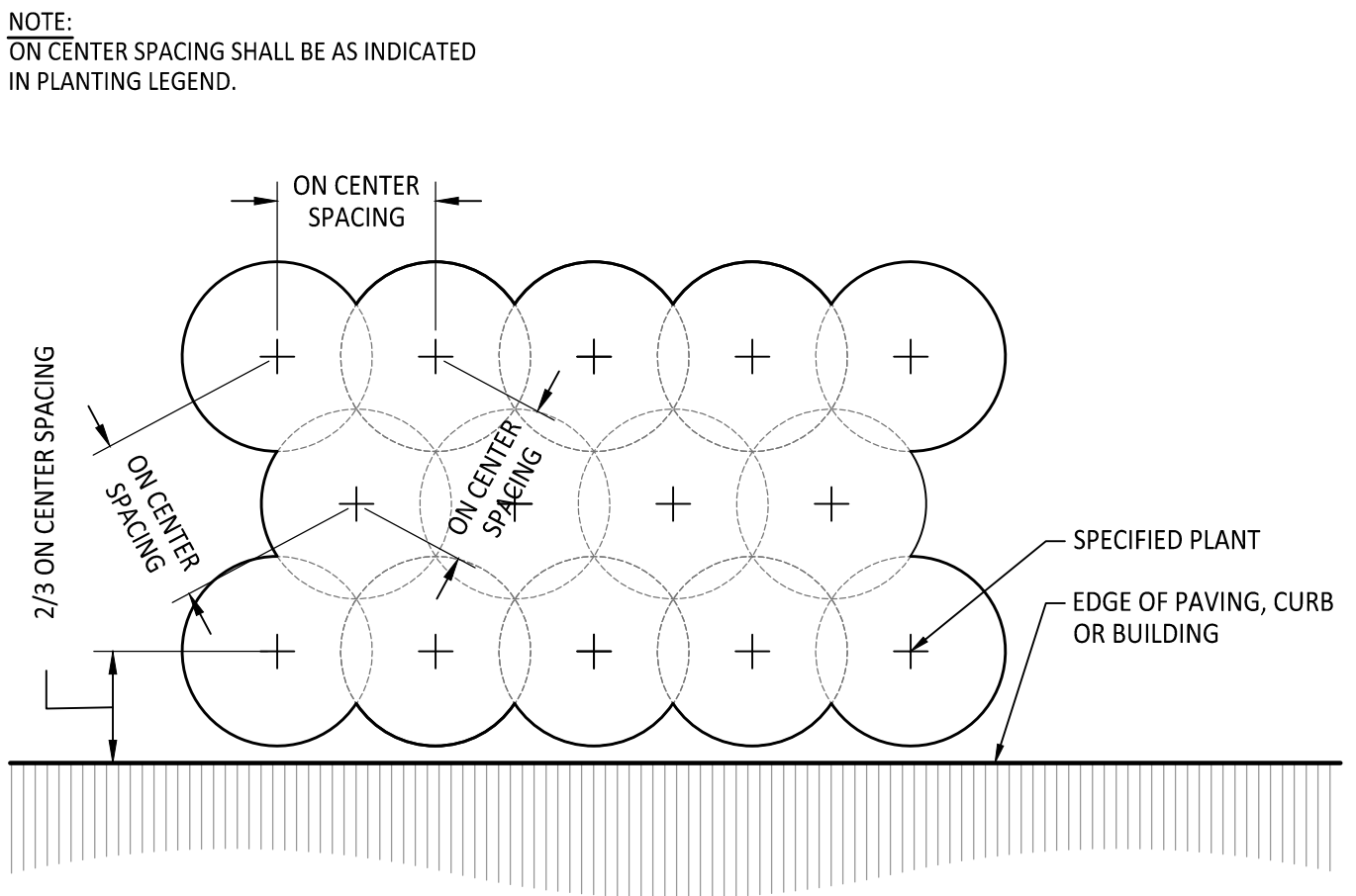
7 TRIANGULAR SPACING Plan NOT TO SCALE
