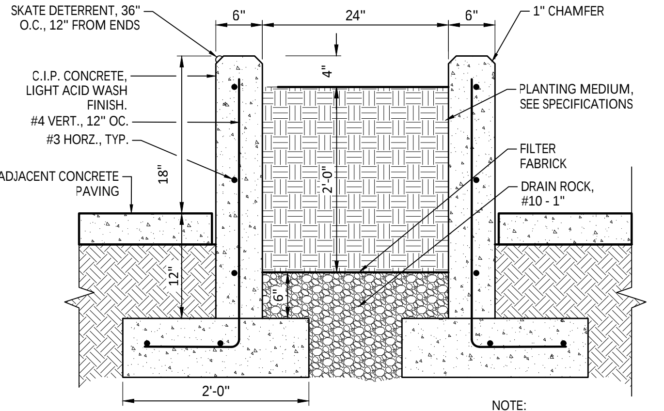
9 PLANTER Section 0 3" 6" 12" SCALE: 1"=1'-0"
