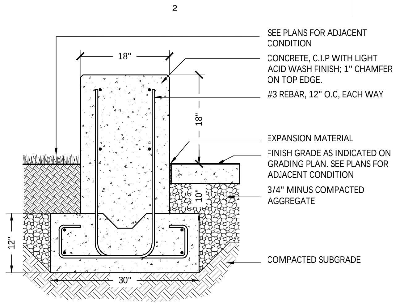
8 SEAT WALL Section 0 3" 6" 12"
