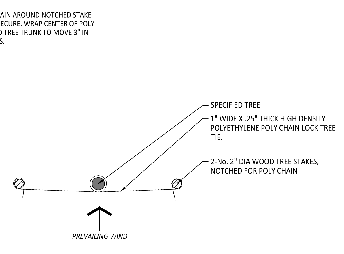
3 TREE STAKING Section NOT TO SCALE
