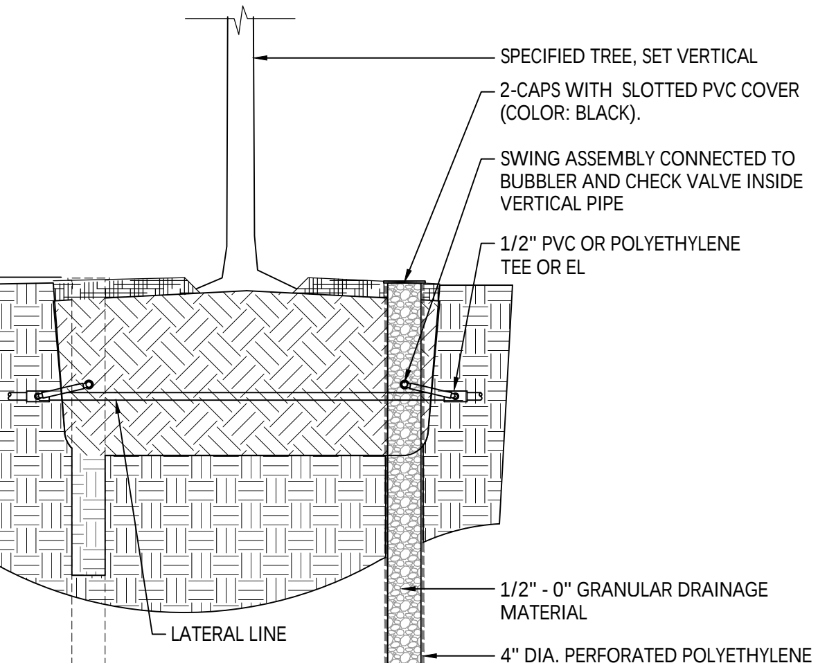
2 DEEP ROOT WATERING Section NTS
